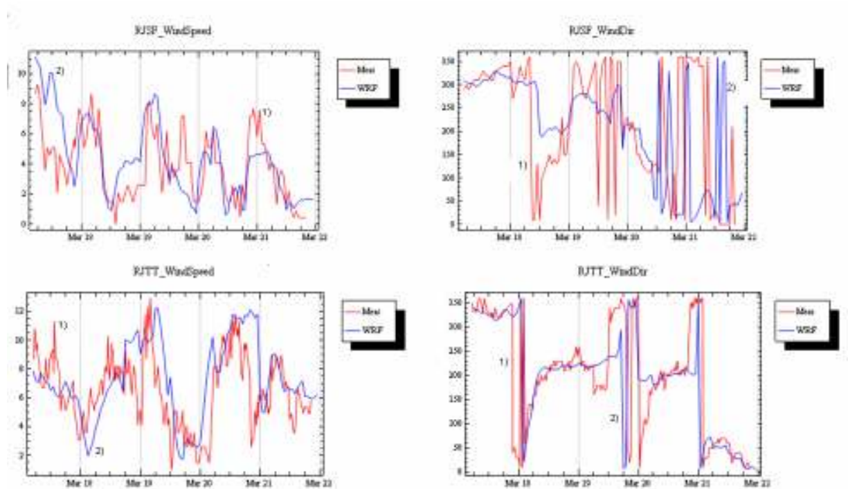
FIG. 2: Comparison of measured (curve 1) and by WRF calculated (curve 2) wind speed (left) and wind direction (right) for the weather stations at Fukushima Airport (top, RJSF) and at Tokyo Airport (bottom, RJTT). Measurements data is taken from Wolfram Mathematica database ( http://www.wolfram.com ).
